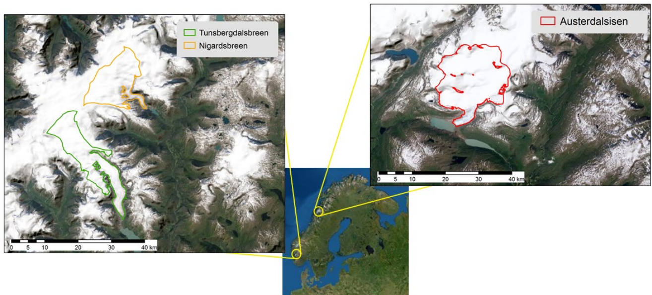
Figure 18. Three largest glaciers in Region 8 – Scandinavia
