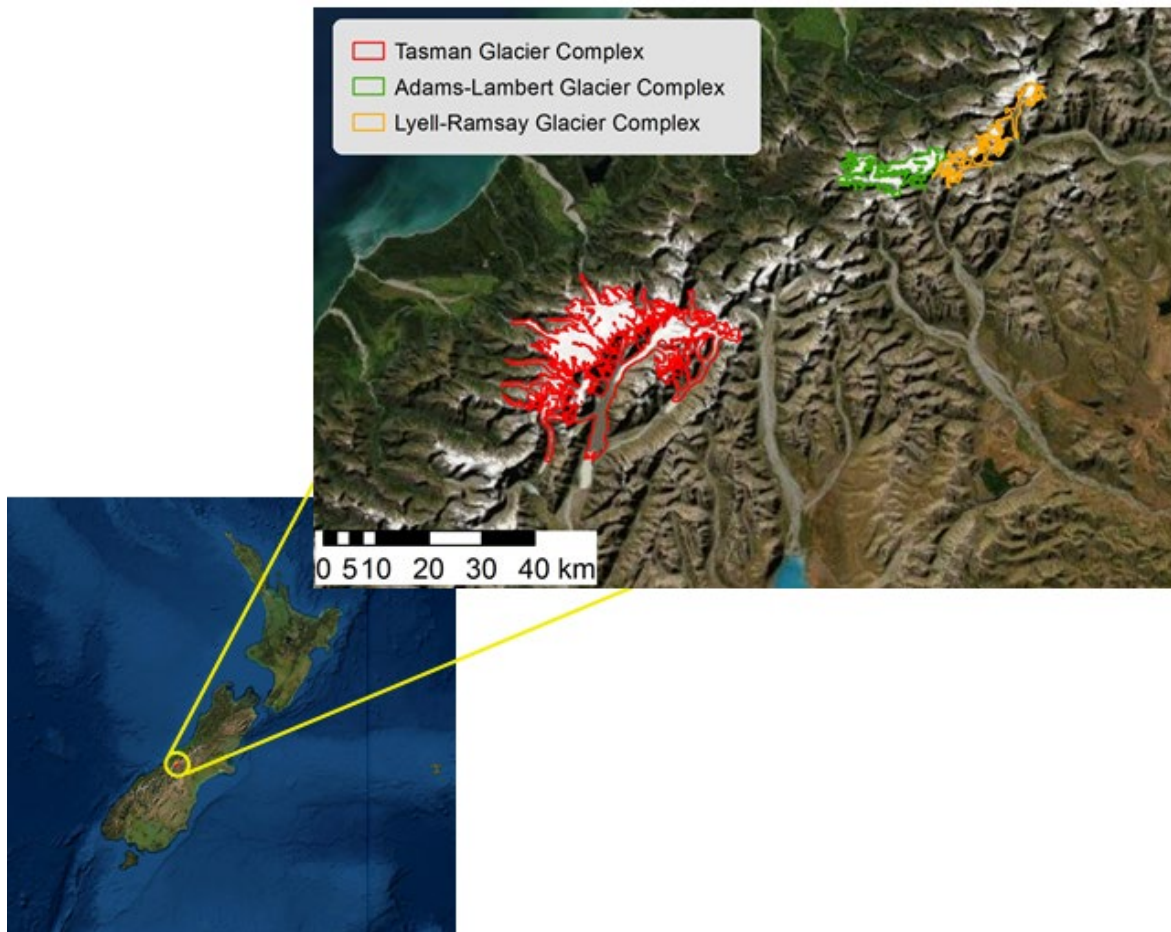
Figure 40. Three largest glacier complexes in Region 18 - New Zealand
