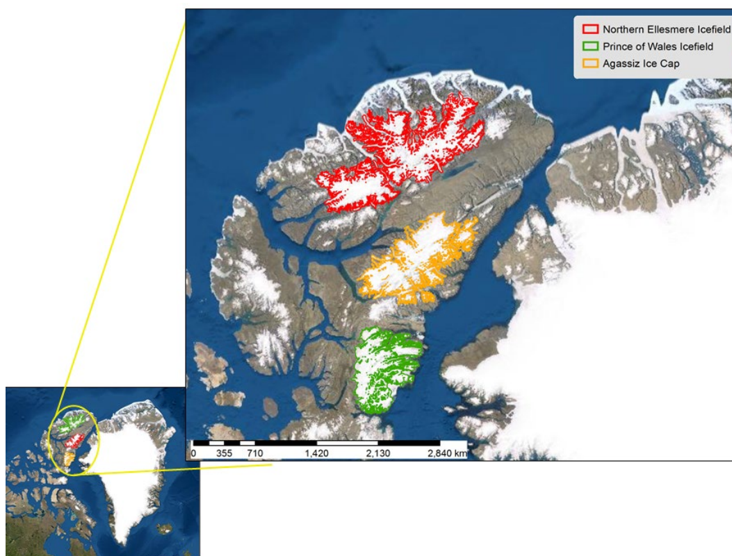
Figure 7. Three largest glacier complexes in Region 3 – Arctic Canada, North
