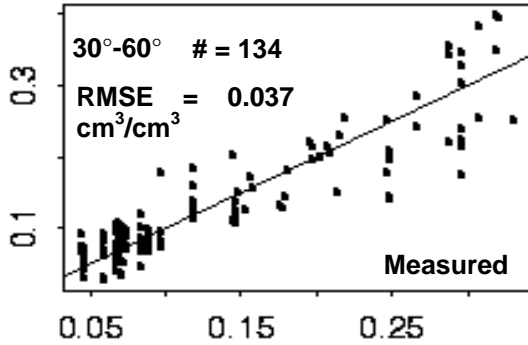
Figure 15. The comparisons between the estimated volumetric soil moisture (y-axis) from two validation data sets and the ground measurements (x-axis).
