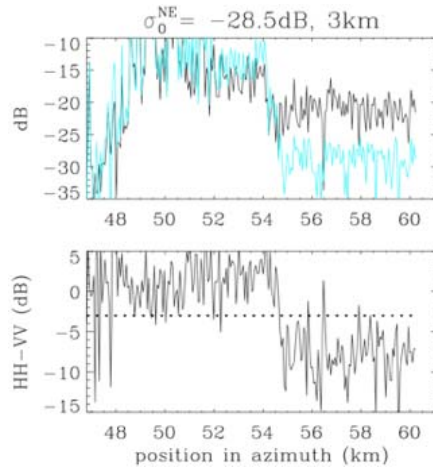
Figure 16 Water body detection tested with a UAVSAR image over the Mono Lake, CA, with the noise level ( \sigma_0^{NE} ) of -28.5 dB. The abscissa is the distance along the 40° incidence angle path (for example, the 60-km mark corresponds to the middle of the lake and the 48 km mark is over land). The top panels show the HH (cyan) and VV (black) co-polarized backscatter. The bottom panels show HH-VV, with the threshold of -3dB shown as a dotted line.
