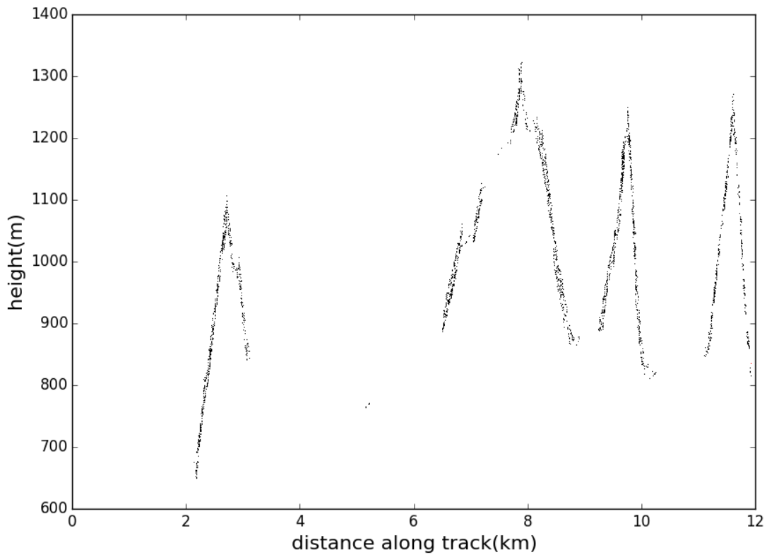
Figure 5-3. Additional Signal Photon Events. Identified via slant histogramming. Black indicates photons found from slant histogramming using the slope from the profile defined by ellipsoidal histogramming.
