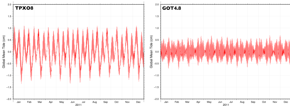
Figure 6-2. One year time series for 2011, of tide values averaged over the global oceans based on a time sequence of 1460, 1°x1° resolution global grids, computed every six hours. TPX08 at left and GOT4.8 at right.
