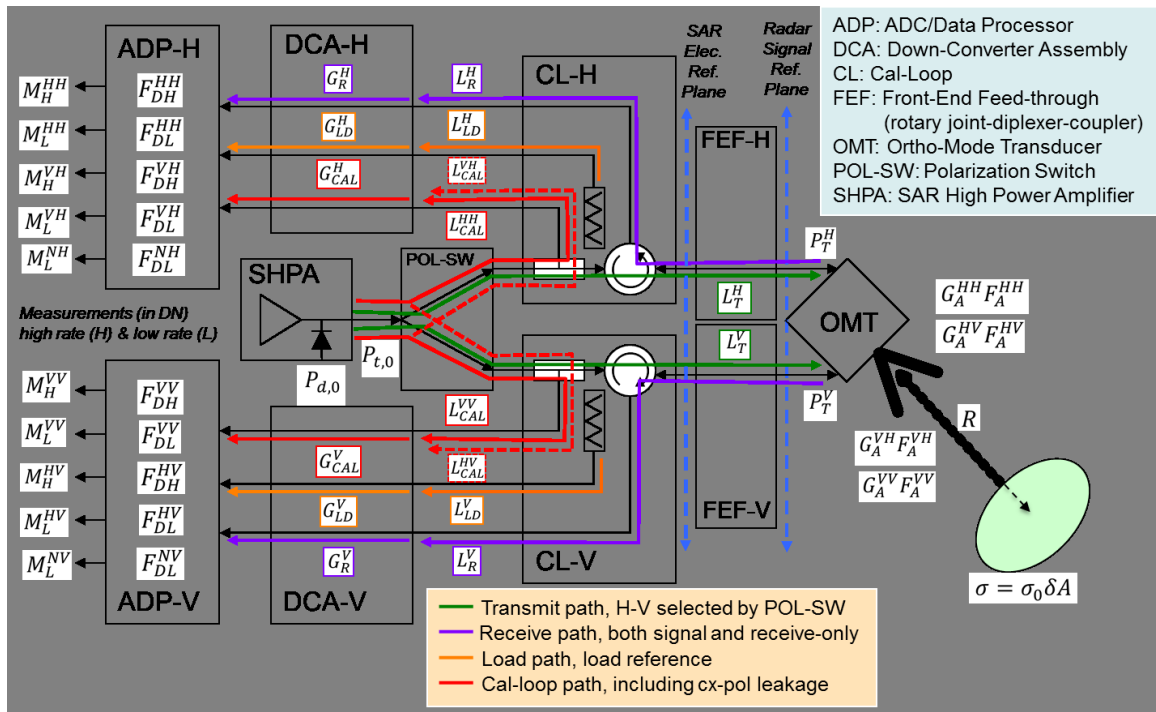
Figure 14: Simplified system diagram showing the loop-back path and the main elements that affect calibration. Passive components with loss are denoted with L, active components with possible gain are denoted with G, and digital processing path gains are denoted as a function F. Different paths are color coded according to the legend.
