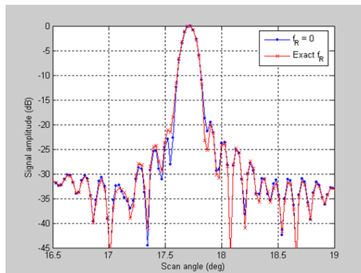
Figure 10: Azimuth cut of the processed image of a point target ( \approx 18^\circ ) with and without f_R in the focusing
