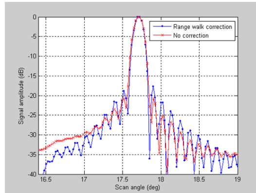
Figure 12: Processed image (azimuth) of a point target near ( 18^\circ ) with and without range walk correction.
