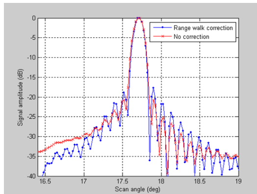
Figure 13: Processed image (azimuth) of a point target near broadside with and without range walk correction.
