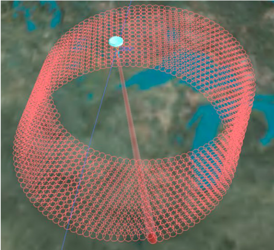
Figure 4: Overlapping conical scans building up as the spacecraft flies a descending orbit track. The scan rotation rate of 14.6 rpm was selected to provide some overlap along the nadir track thus filling in the 1000 km wide swath with radar measurements.
