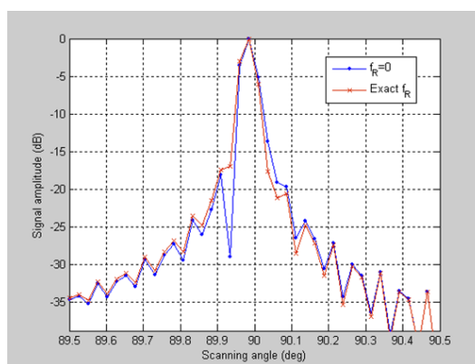
Figure 11: Azimuth cut of the processed image of a point target ( \approx 18^\circ ) with and without f_R in the focusing
